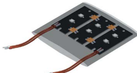
LED MC-PCB
